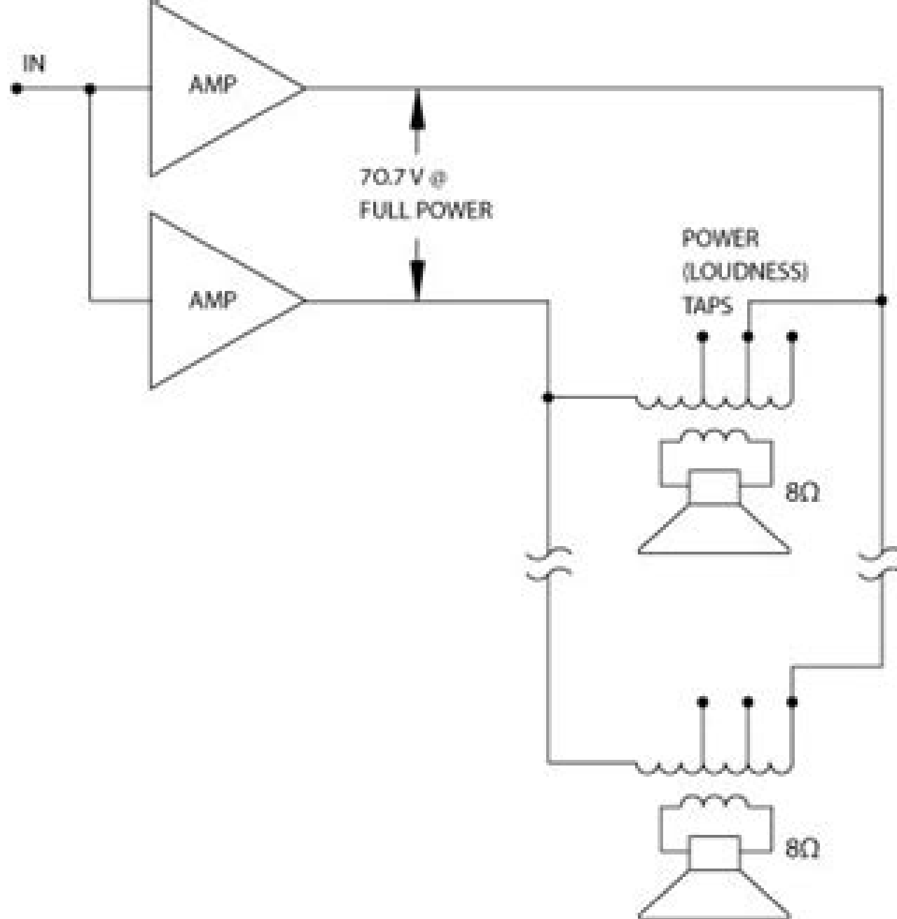
Figure 3. 70.7V Direct-Drive Constant-Voltage Distribution System
