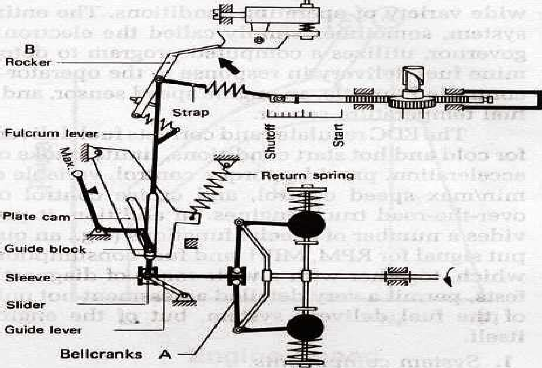
FIGURE 20.28 RQV governor torque control (courtesy Robert Bosch GmbH).
