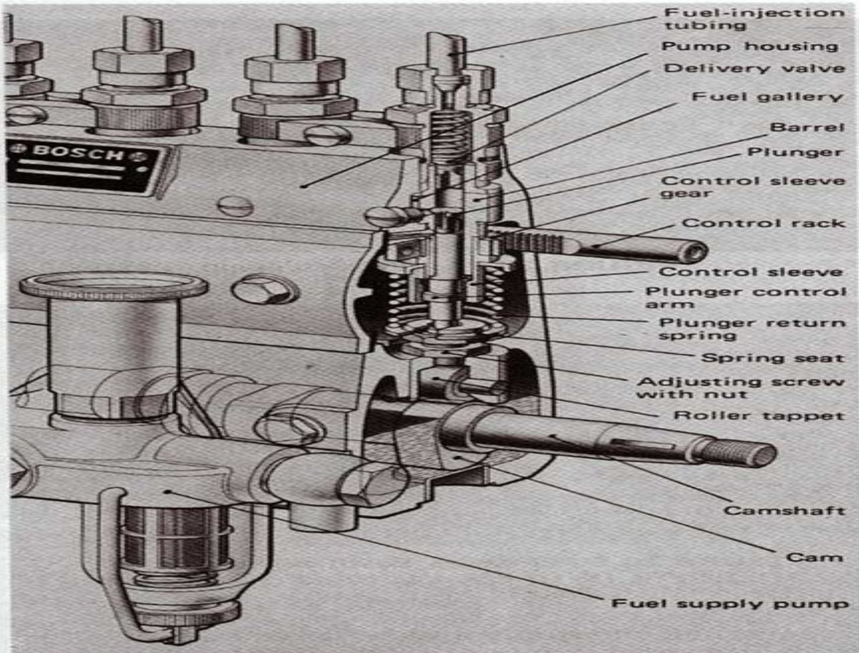
FIGURE 20.9 A series in-line pump (courtesy Robert Bosch GmbH).
