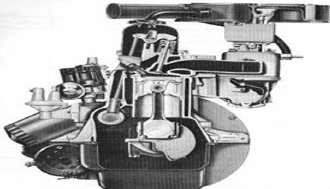
SECTIONAL VIEW OF ENGINE ASSEMBLY
