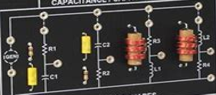
RL / RL WAVESHAPES
