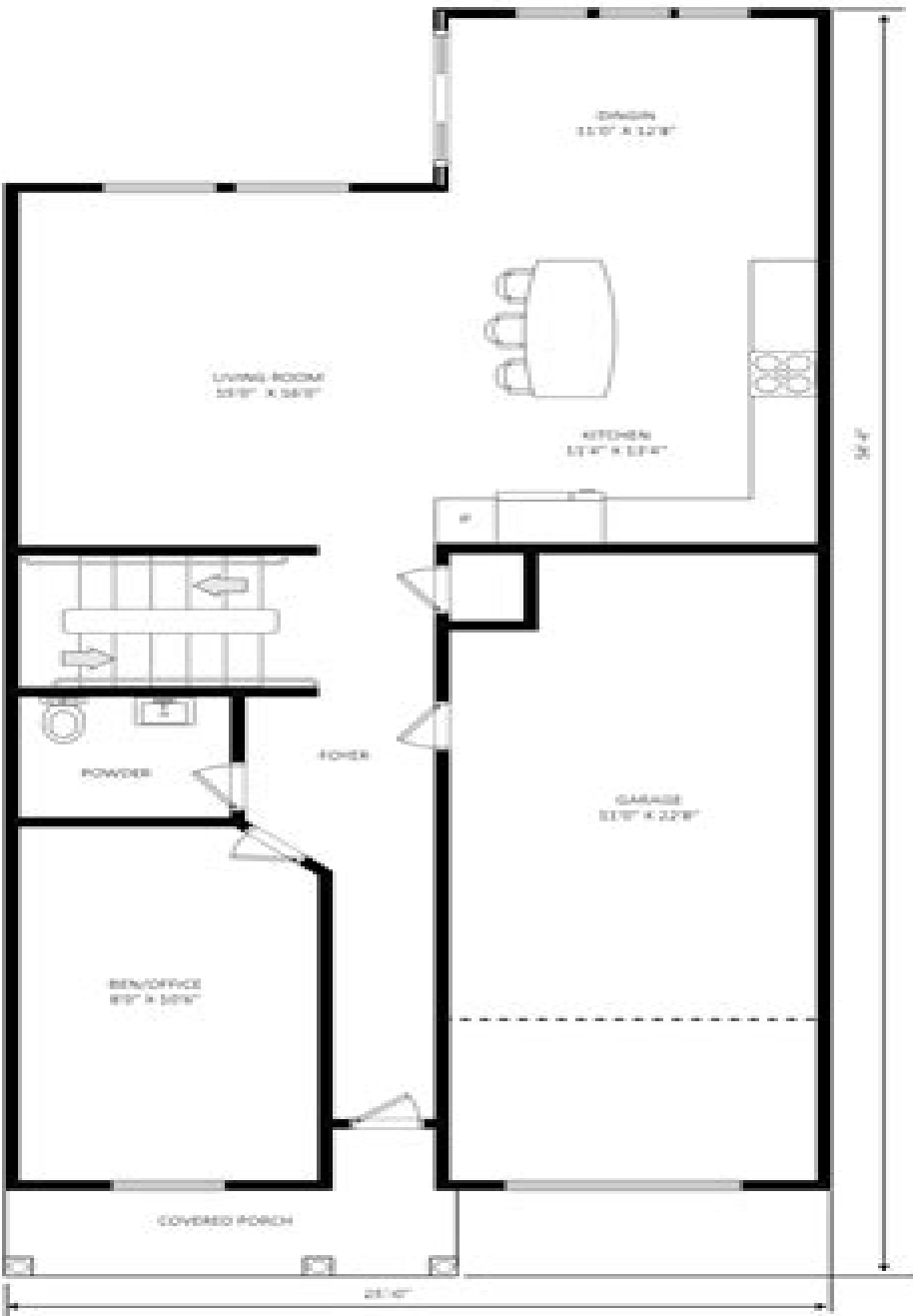
1ST FLOOR PLAN GROSS FLOOR AREA : 886 SQ.FT.
