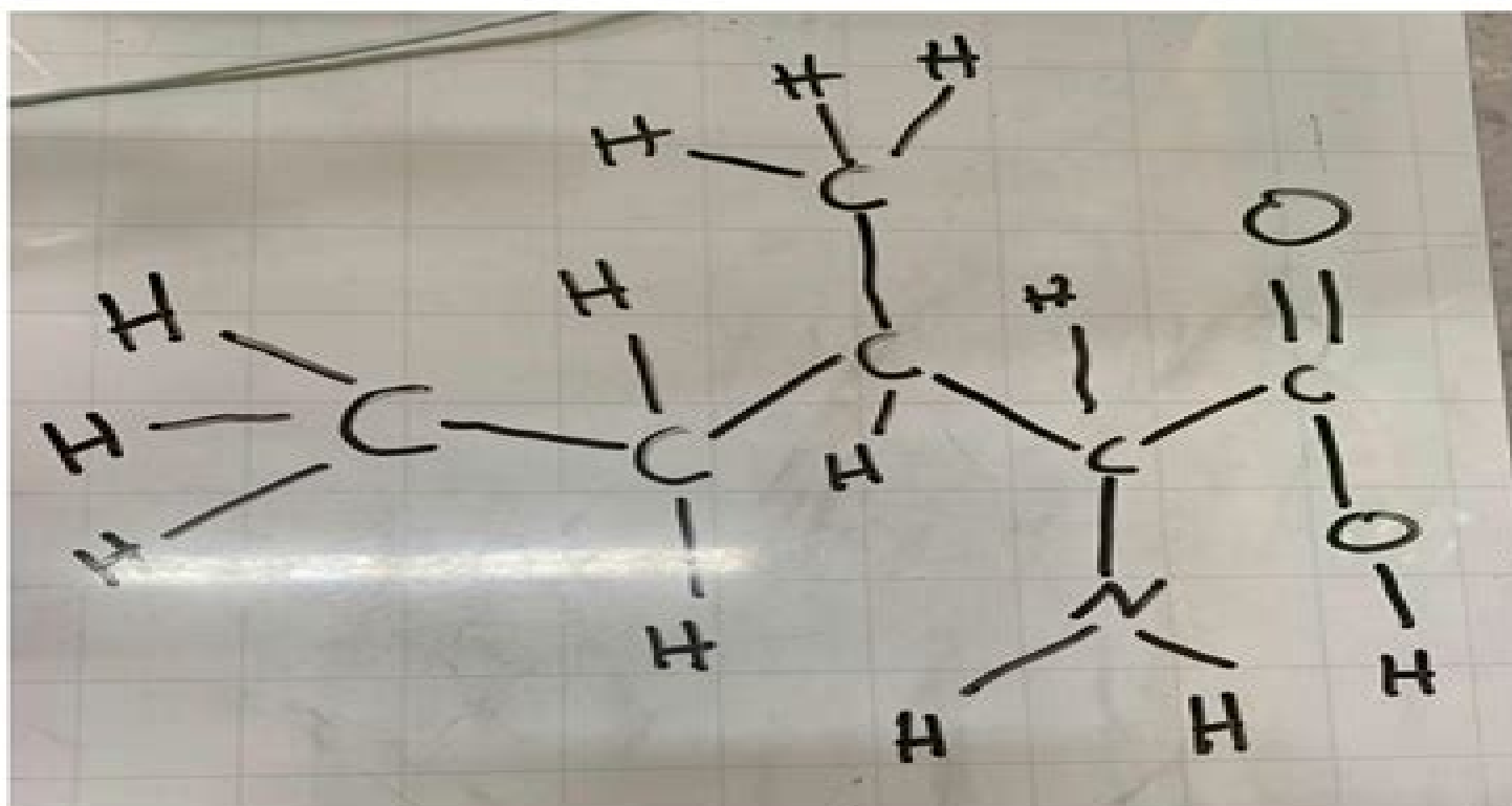
Isoleucine
