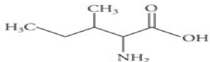
Isoleucine
