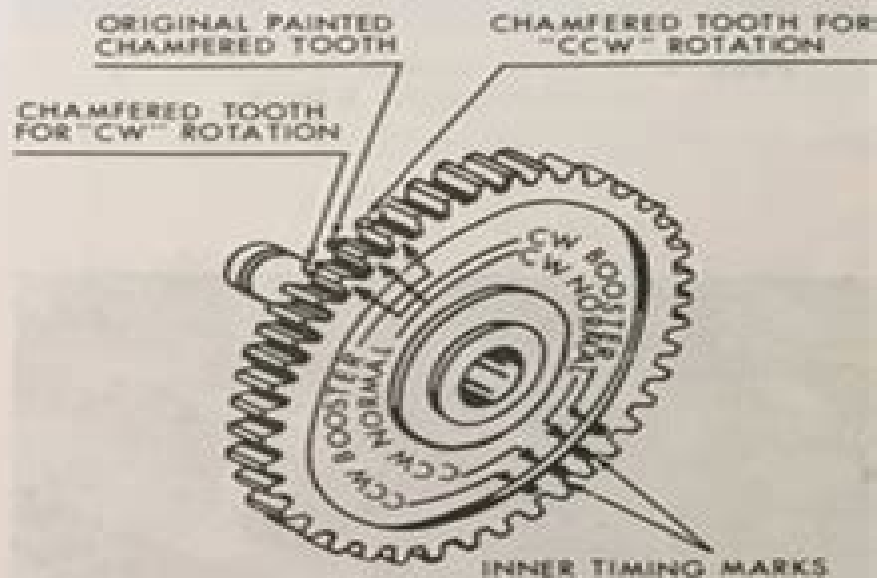
Figure 2-31. Six Cylinder Gear
