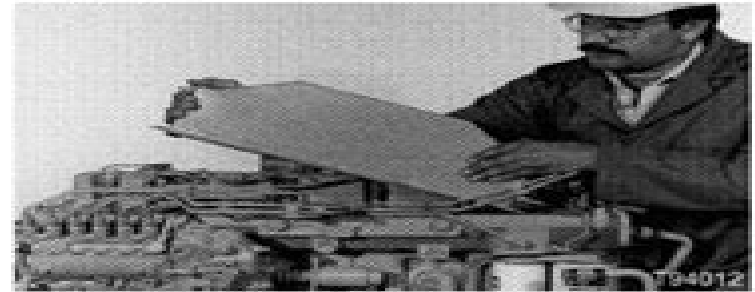
Remove the bolts and aftercooler. Discard the gasket. Clean the gasket surfaces. Inspect the housing and core for damage.
