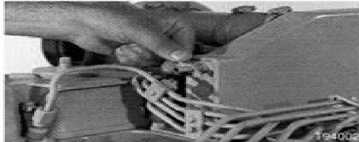
Drain the coolant from the engine. Open the air vent valve on the aftercooler to help drain the coolant.
