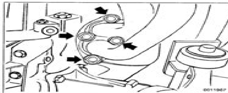
Fig. 6. Front exhaust pipe to exhaust mounting nuts (arrows), as viewed from below on 4-cylinder engine.
