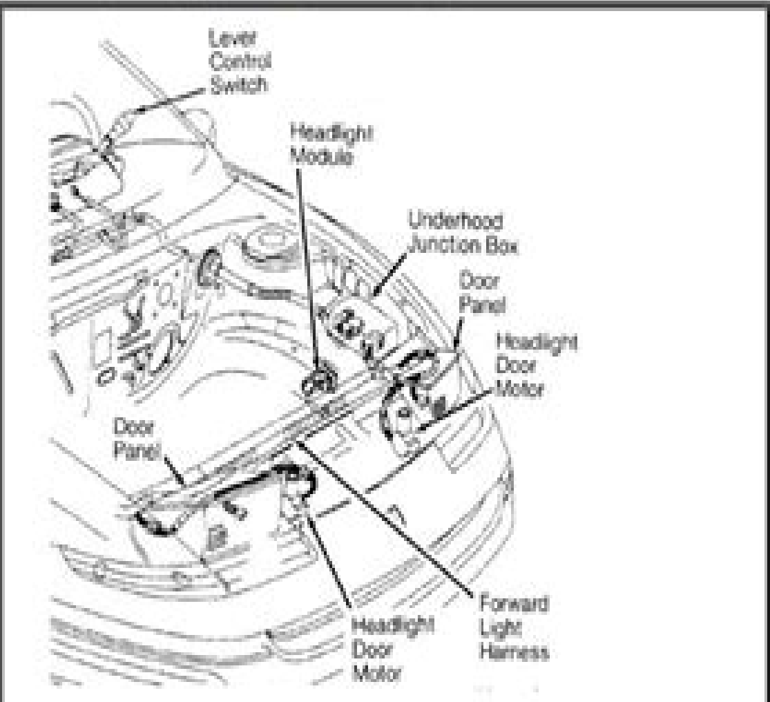
Fig. 4. Headlight Door Component Location (SCL & SCL) Courtesy of GENERAL MOTORS CORP.
