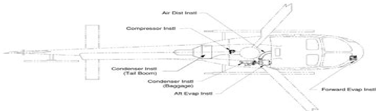
Figure 4-2 – Layout of AS350 Air Conditioning System
