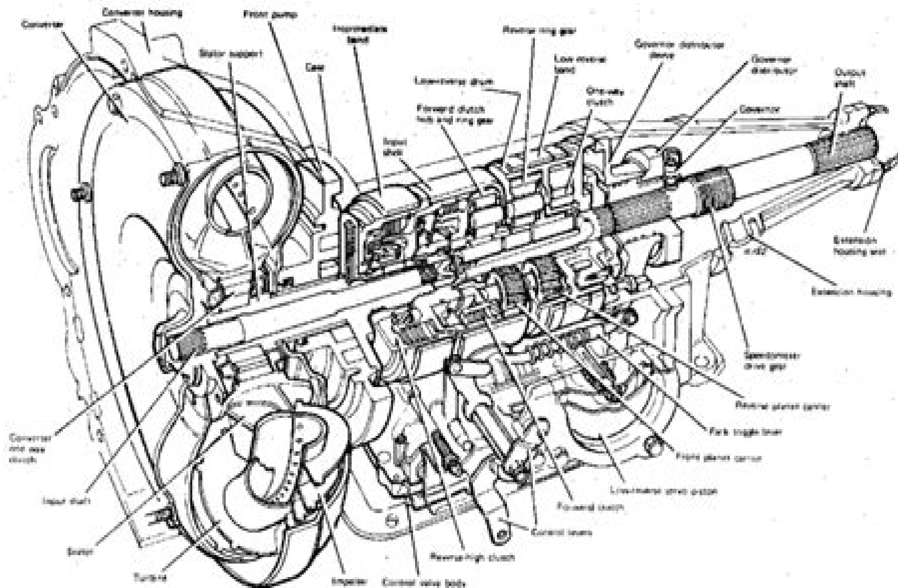
The Ranger Station - Exploded View Of 4R23W Transmission
