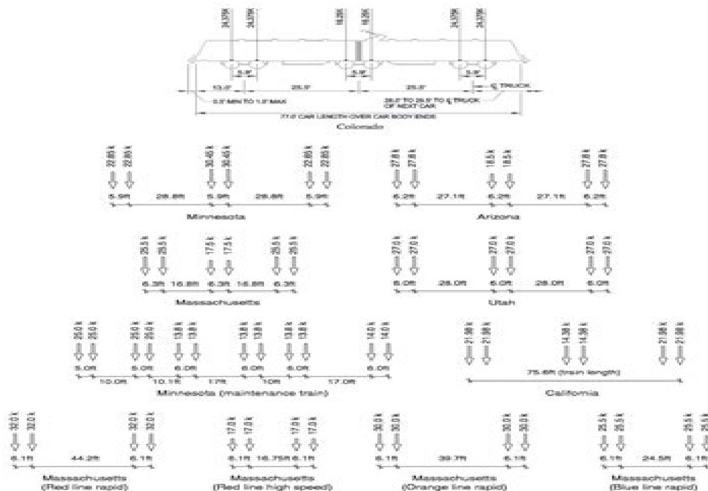
Figure 2.1. Various design live loads for light rail transit (axle load).
