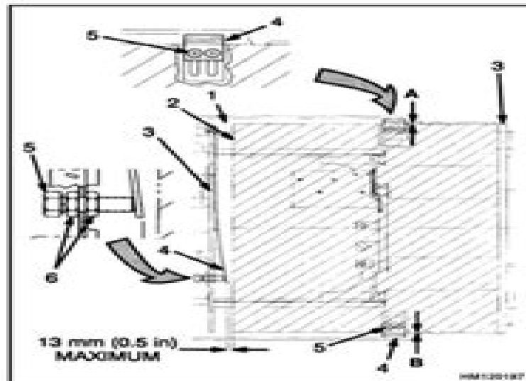
Figure 4. Spacers of Battery Compartment
