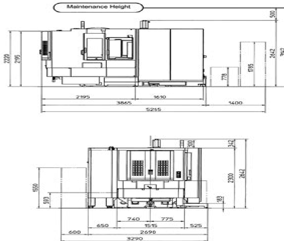
Figure 2.1 Side and Front View of Machine (Tool Magazine A40/A60 and Left-Discharge Conveyor Specs.)
