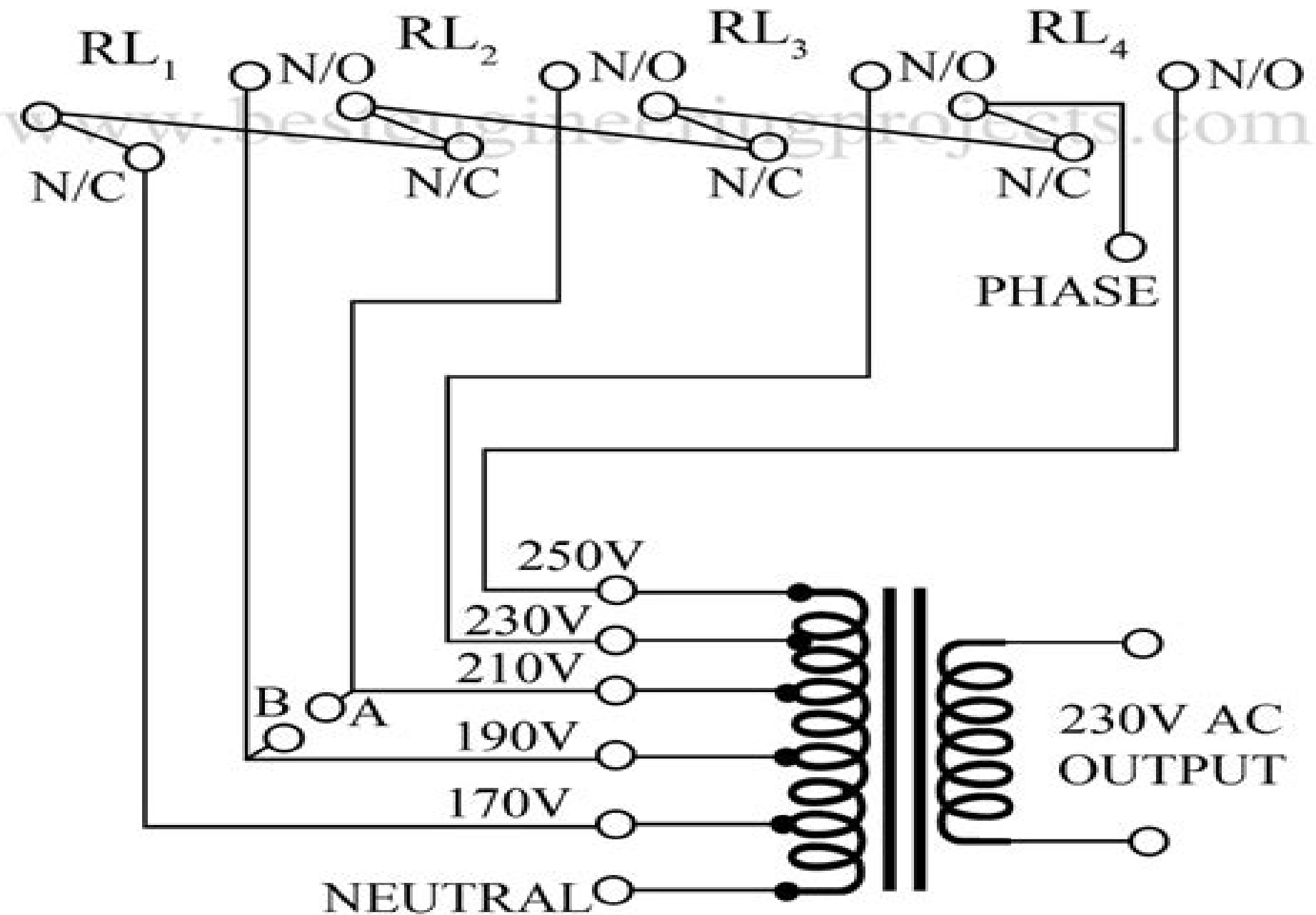
Figure 2: Relay and Transformer Connection Diagram
