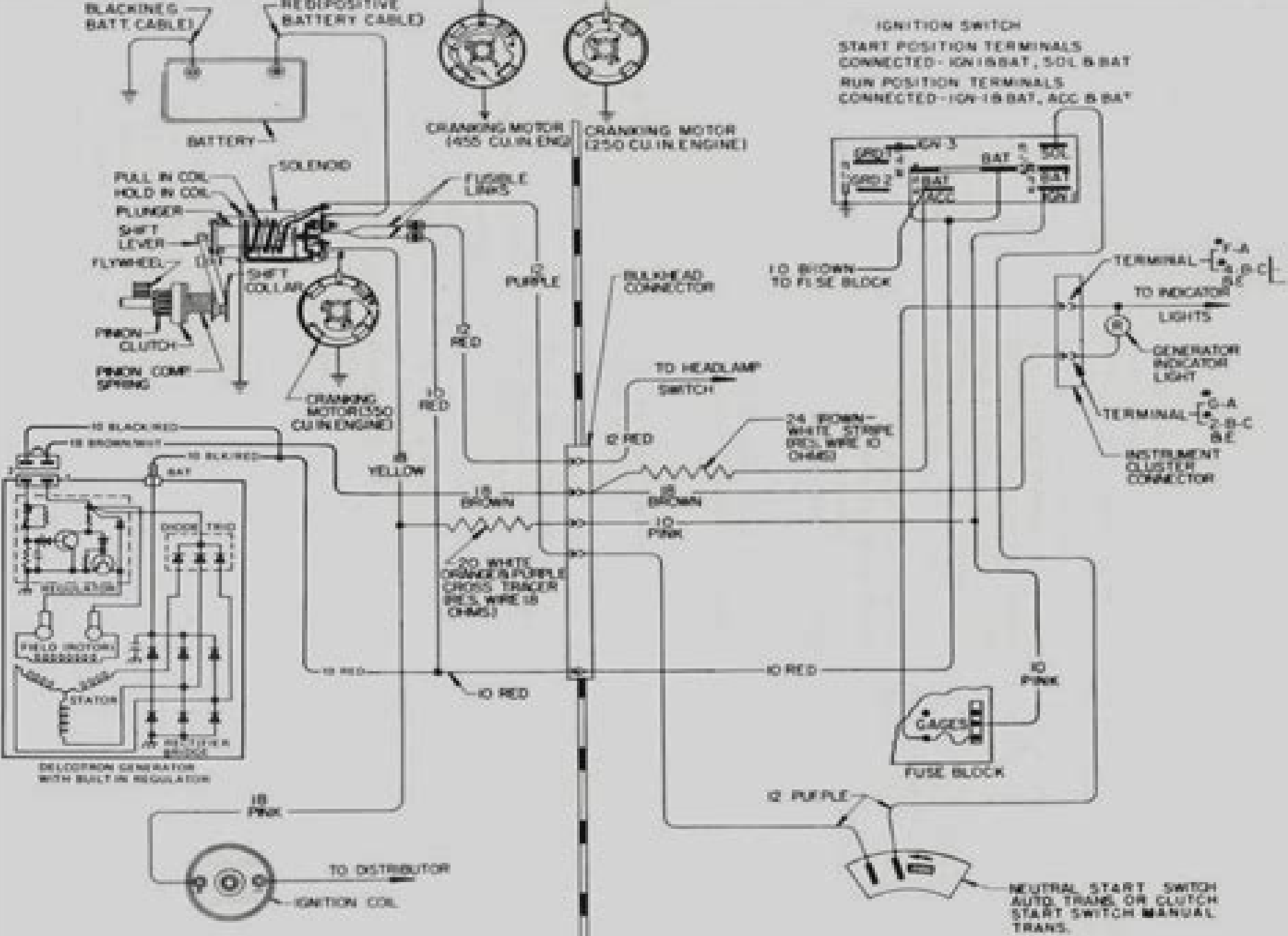
PART OF ENGINE WIRING HARNESS
