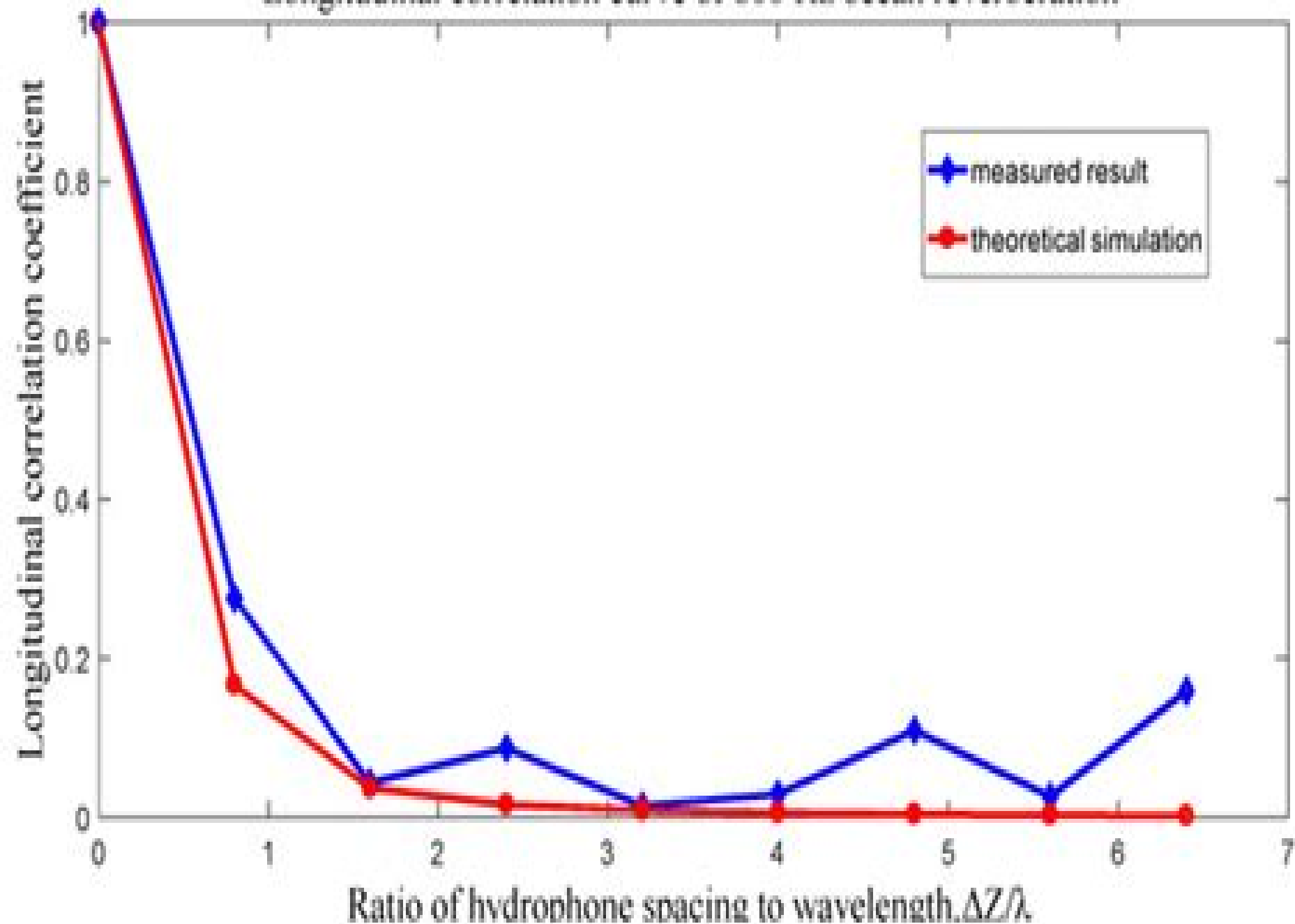
Longitudinal correlation curve of 800 Hz ocean reverberation
