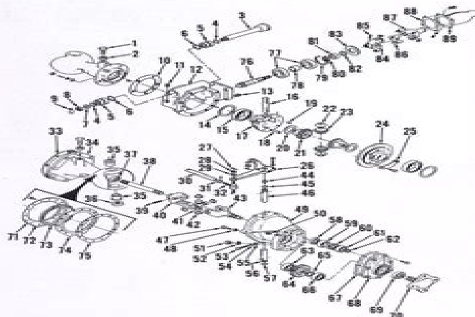
Fig. 3—Exploded view of front-wheel drive axle used on Model B510SD. Front-wheel drive axle used on Models B610SD, B6100HST-D and B710SD is similar except for pinion gear assembly and location of differential drain plug (see Fig. 4).
