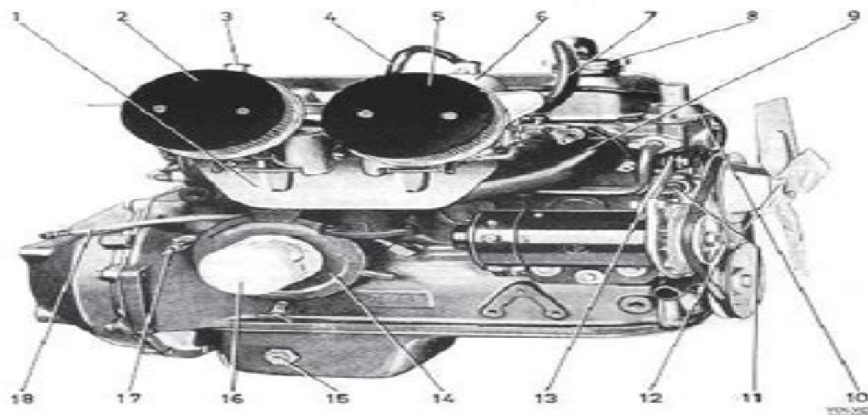
Fig. 3. The engine viewed from the right (Oil cooler only on B 18 B early prod.)
