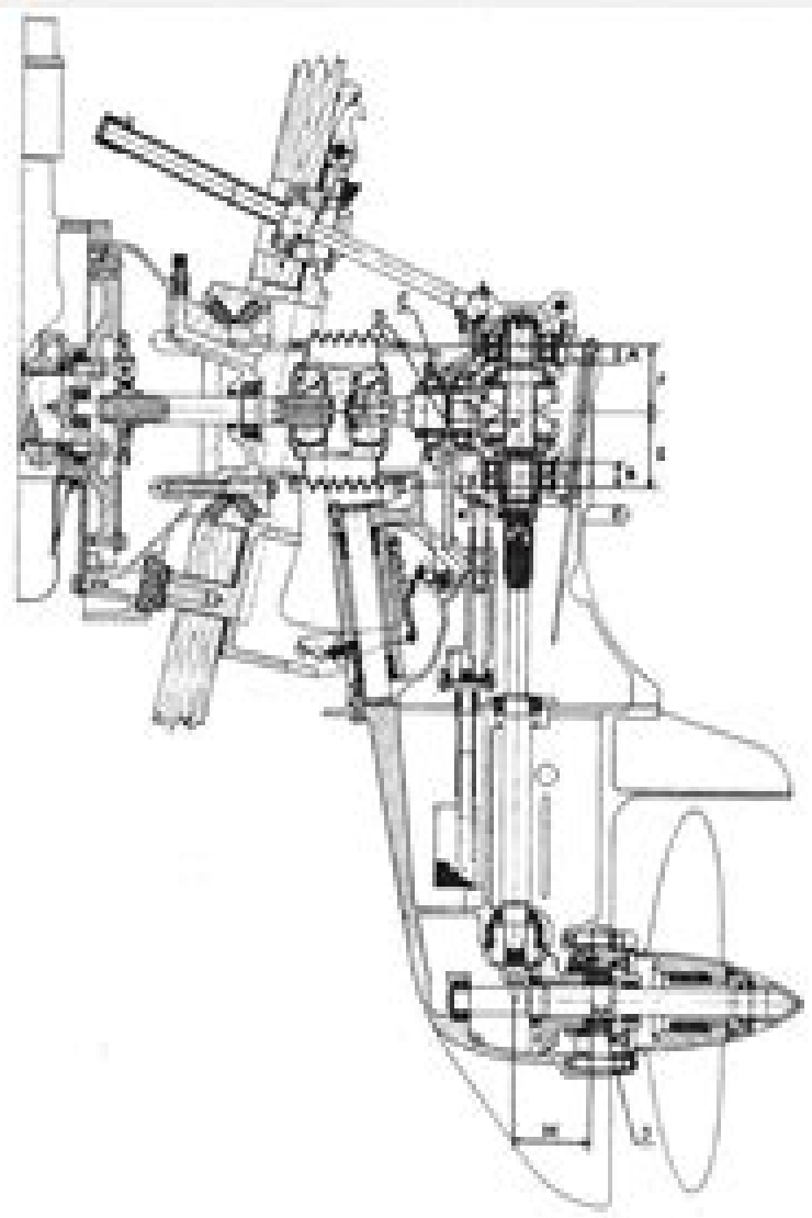
Fig. 40 Assembly drawing
