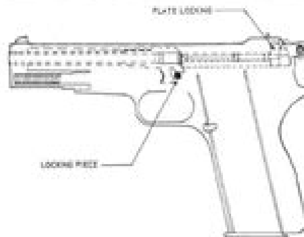
Figure 4 - Lateral Movement of Slide
