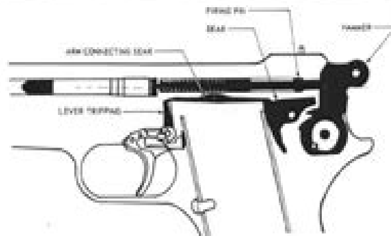
Figure 3 - Trigger Mechanism - Trigger Squared
