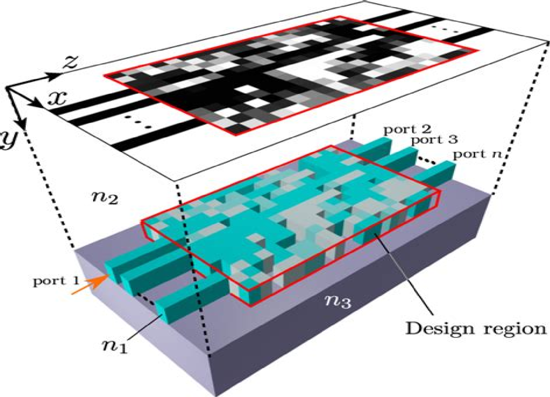
FIG. 1 Design model of optical waveguide devices
