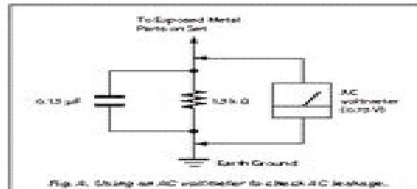
Fig. A. Using an AC voltmeter to check A/C leakage.
