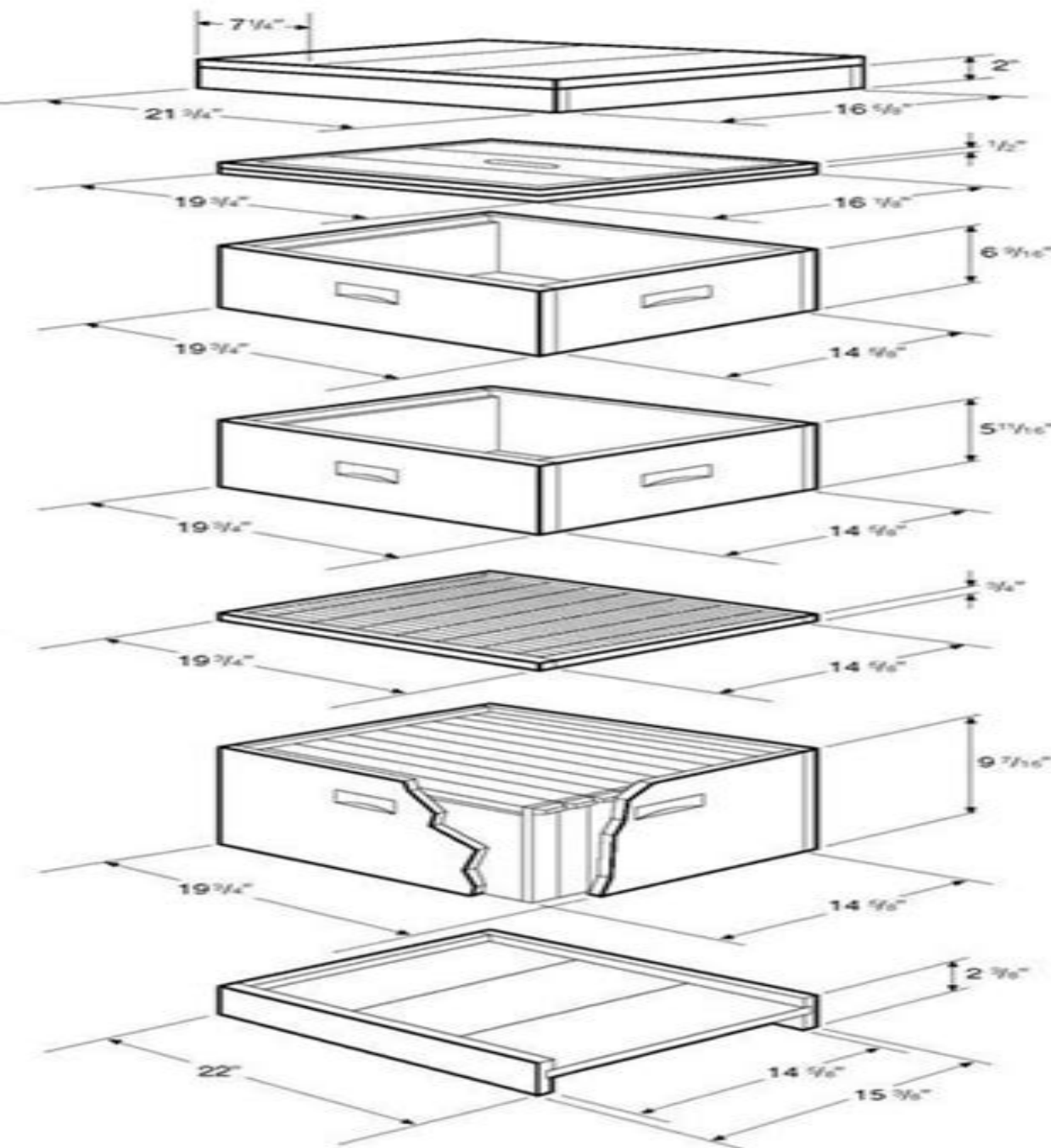
Figure 21. The parts of a modern honey bee hive.
