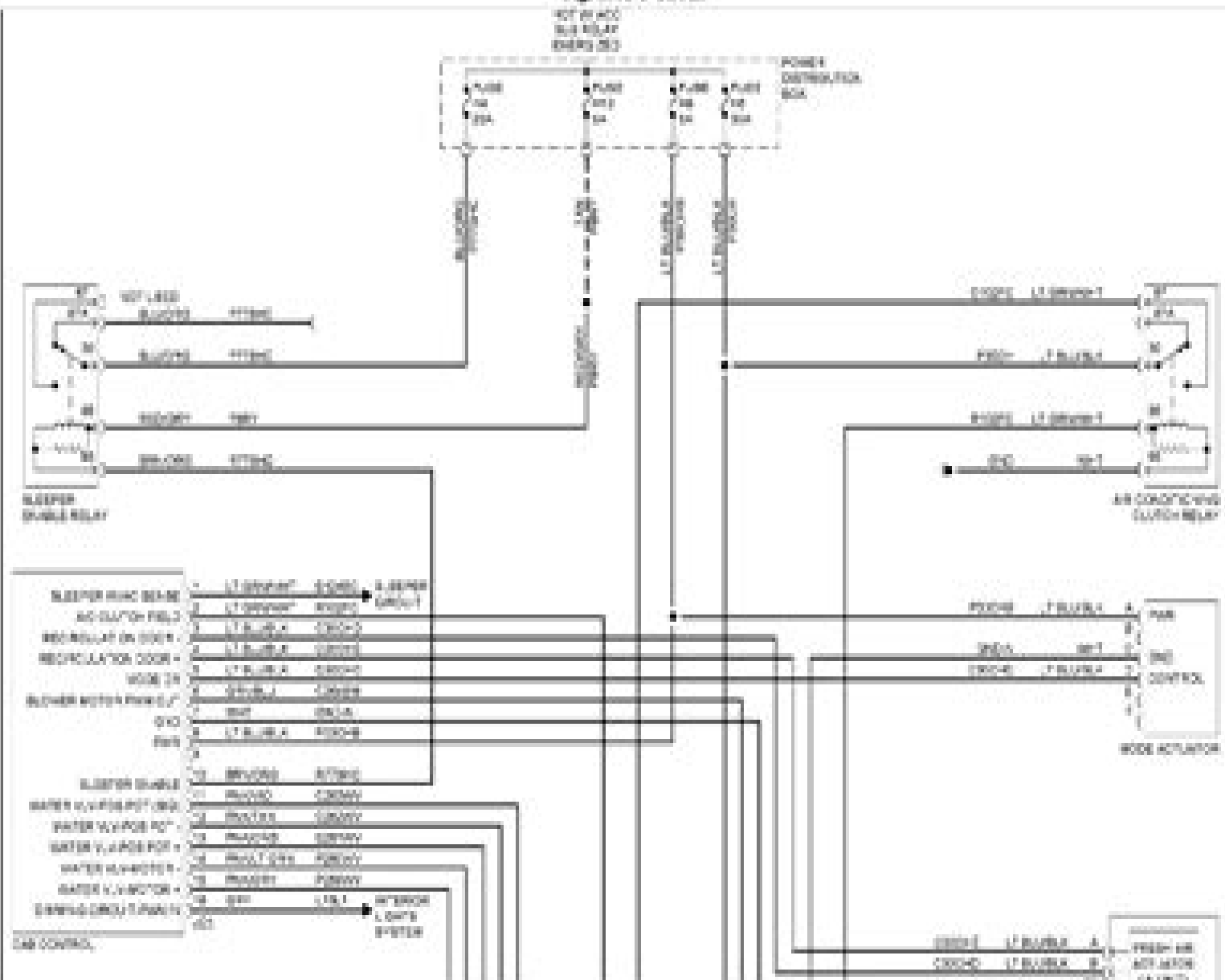
Fig. 1: AC Circuit
