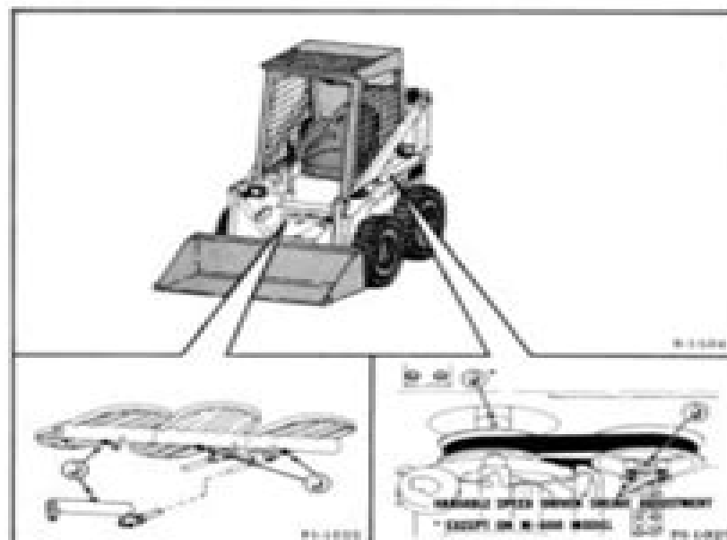
Fig. 5-2 Loader Lubrication
