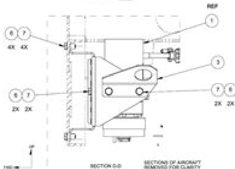
SECTION D-D SECTIONS OF AIRCRAFT REMOVED FOR CLARITY
