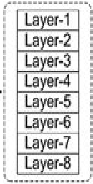
DNN
