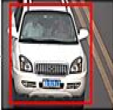
Vehicle Detection
