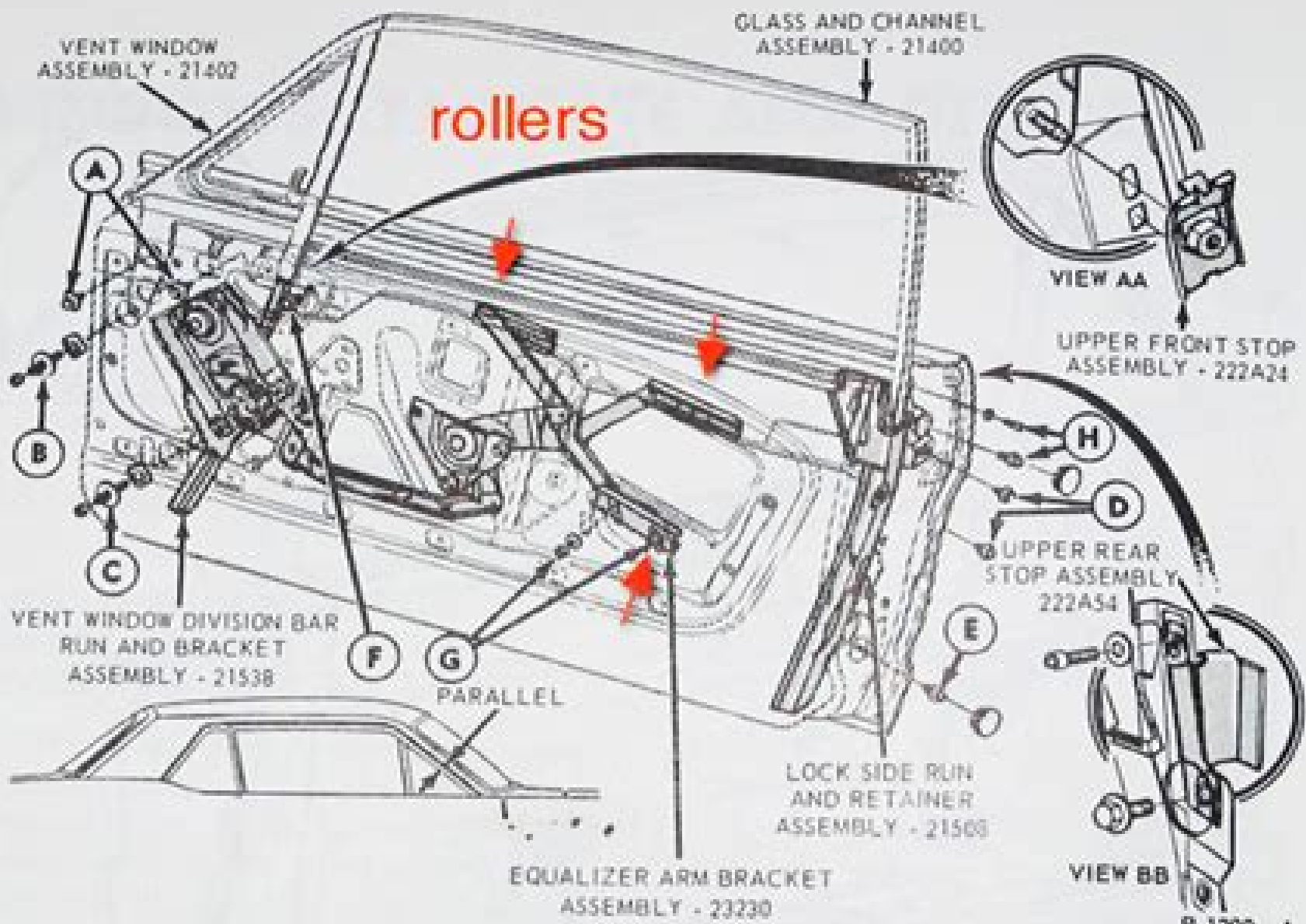
FIG. 17-1. VENT WINDOW ASSEMBLY
