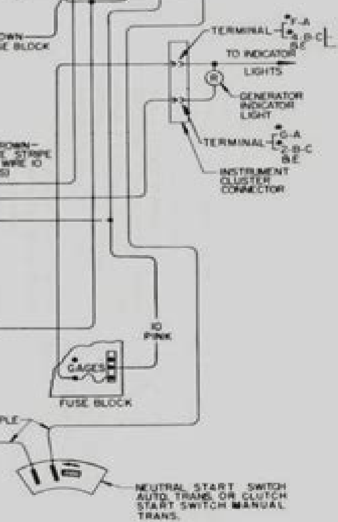
PART OF INSTRUMENT PANEL WIRING HARNESS
