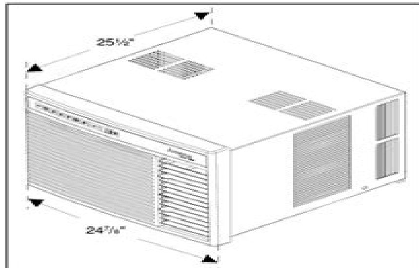
Air Conditioner Dimensions (with chassis installed)
