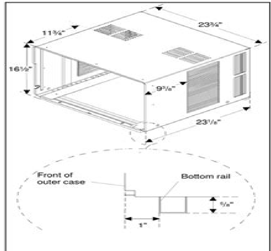
Outer Case Dimensions (chassis removed)
