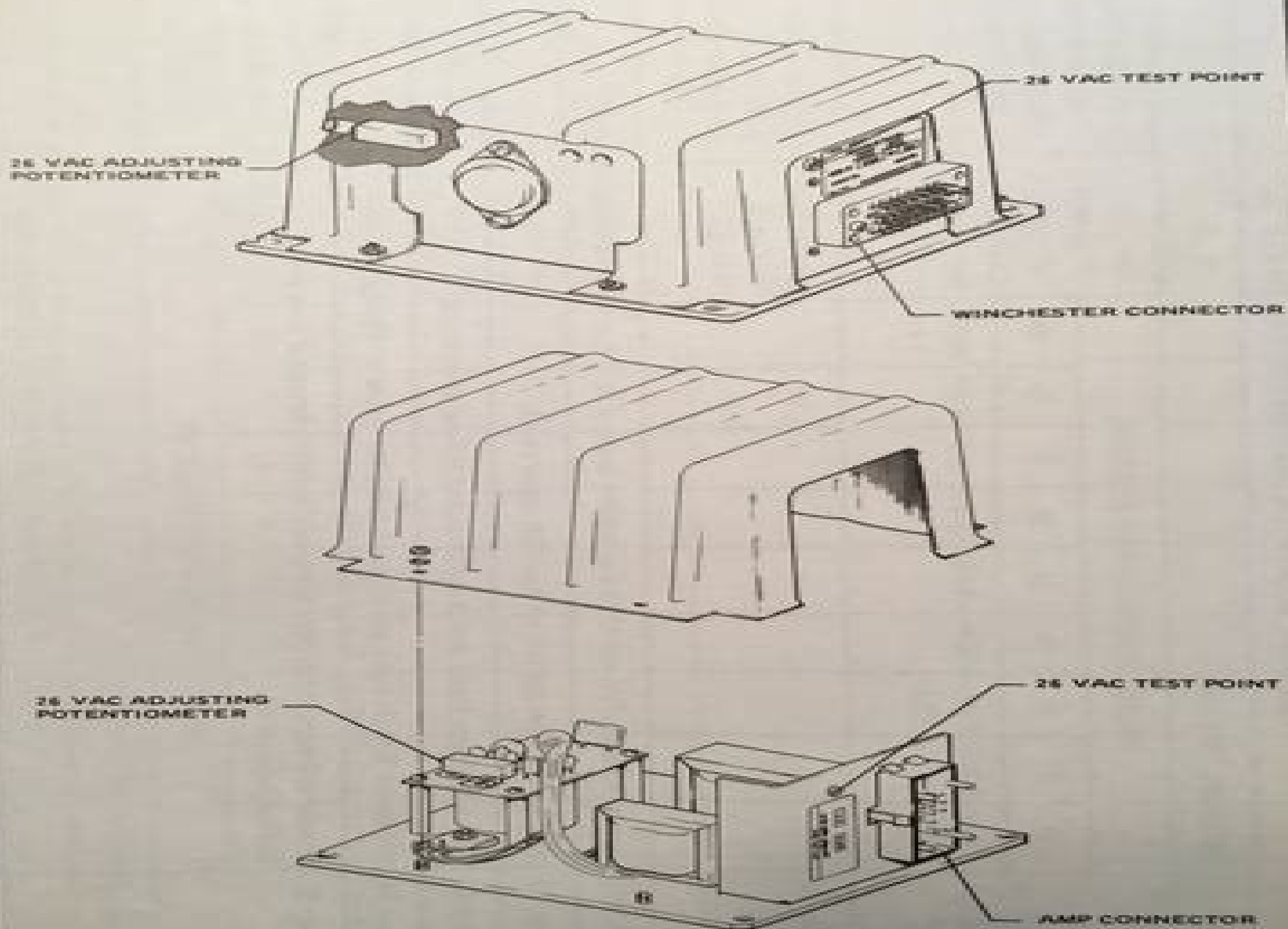
Figure 4-2. AlluMatic V Power Supply
