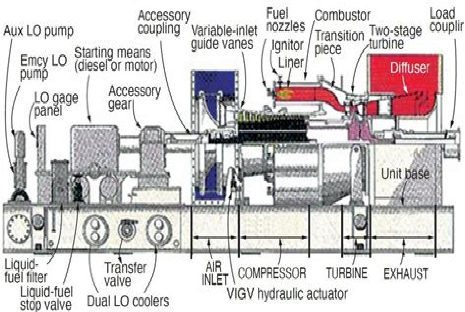
1. MS5001 gas turbine (right-side view) identifies auxiliaries and their locations on the accessory base and turbine base
