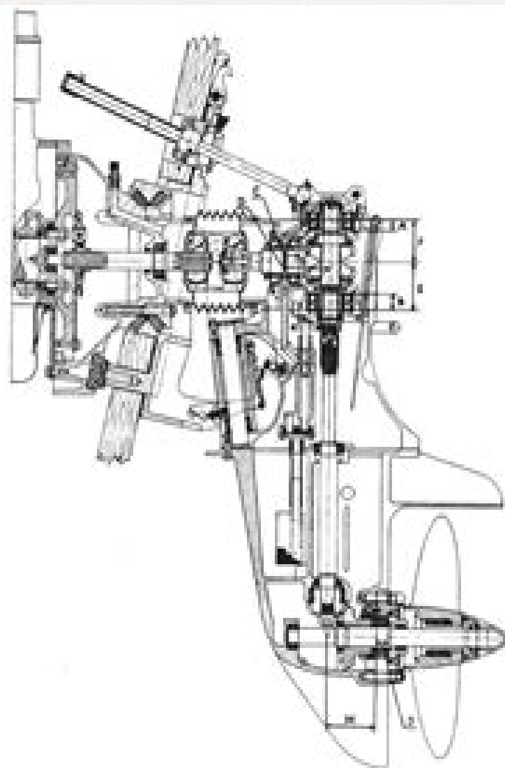
Fig. 40 Assembly drawing
