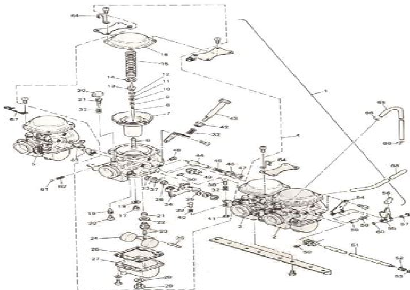
Bank of four Mikuni BS34-11 2H7-00 CD carburetors as fitted to Yamaha XS 1100
