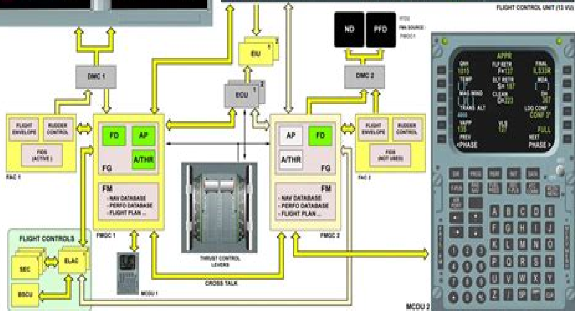
FLIGHT CONTROL UNIT (13 VU)
