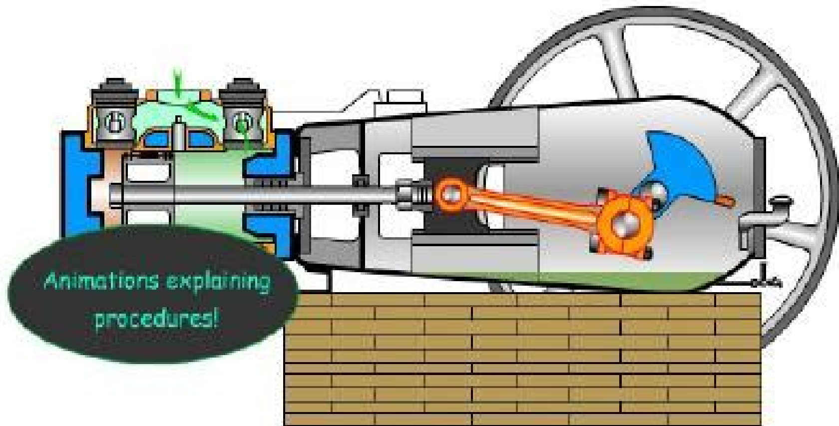
A HORIZONTAL SINGLE STAGE DOUBLE ACTING COMPRESSOR
