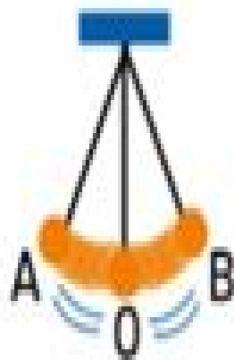
Oscillatory Motion
