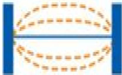
Vibratory Motion
