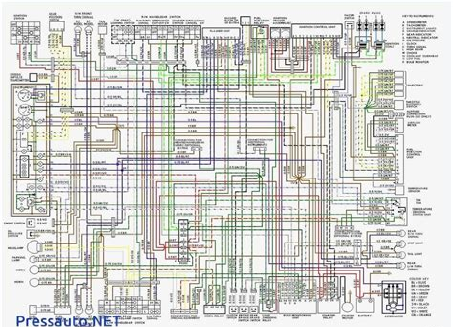
Wiring Diagram - early 1900 RS and RT model
