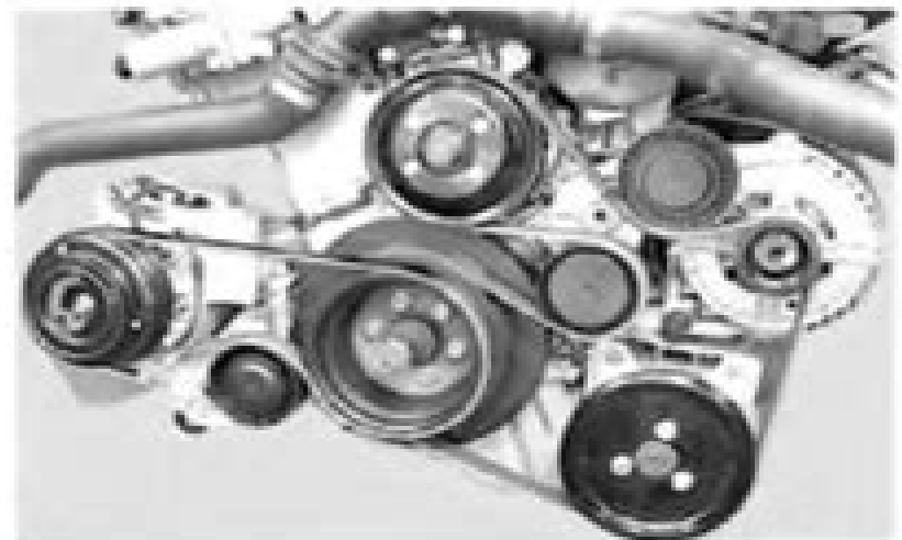
Timing Drive Belt Running Without Auxiliary Tensioning Pulley (M52, M54 & S52) BMW OF NORTH AMERICA, INC.
