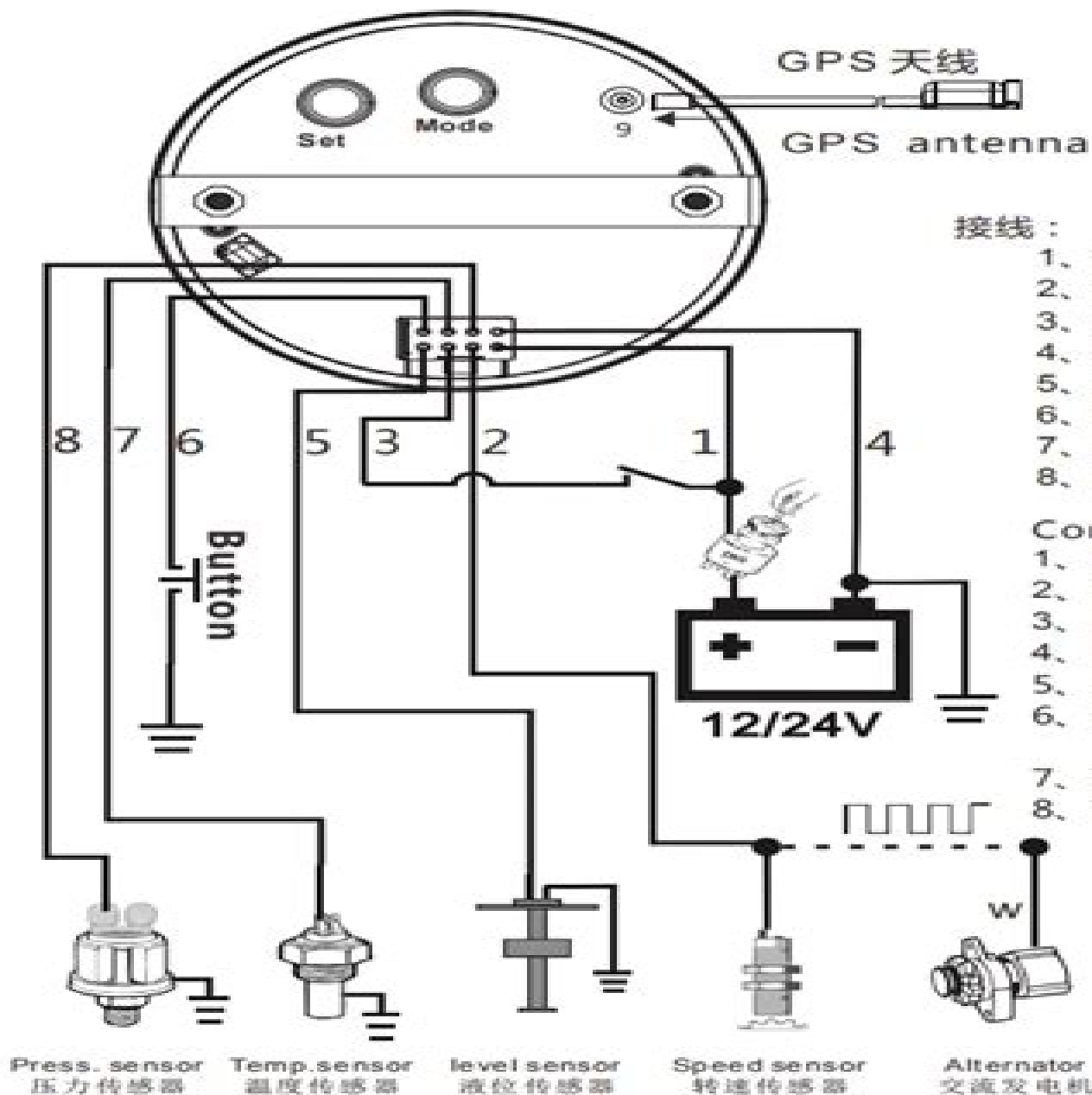
E 接线图 Wires Connecting
