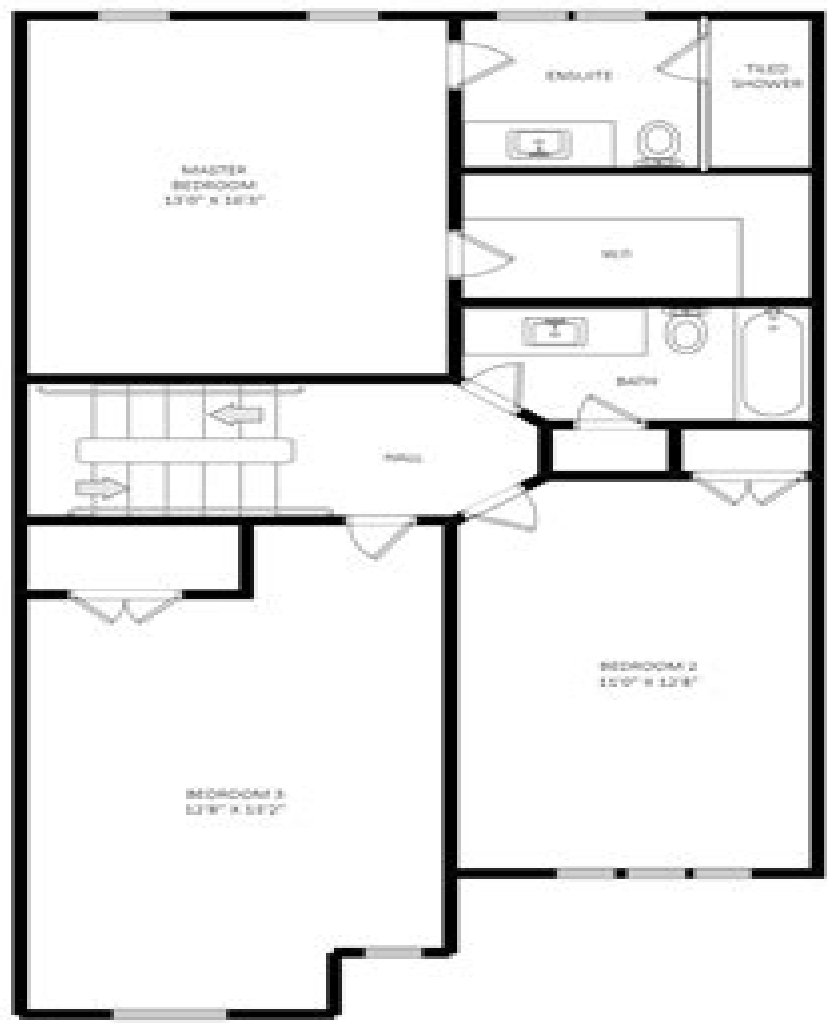
2ND FLOOR PLAN GROSS FLOOR AREA: 888 SQ.FT.
