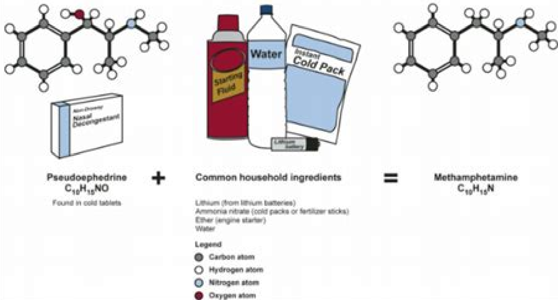
Figure 1: Conversion of PSE to Meth
