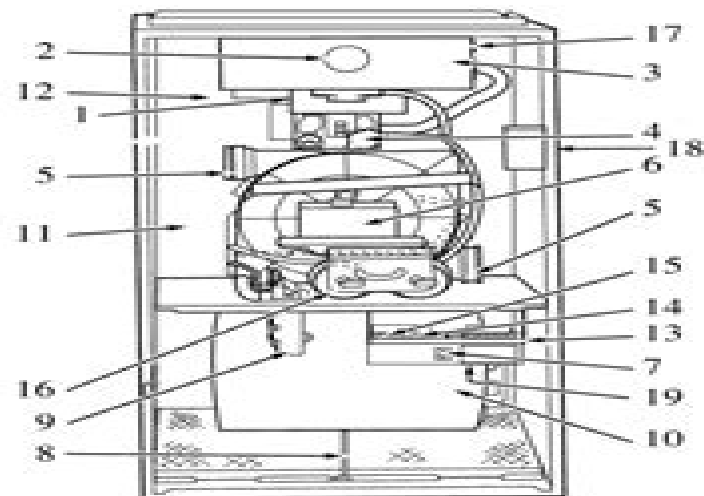
MODEL 355MAV FURNACE (UPFLOW POSITION)
