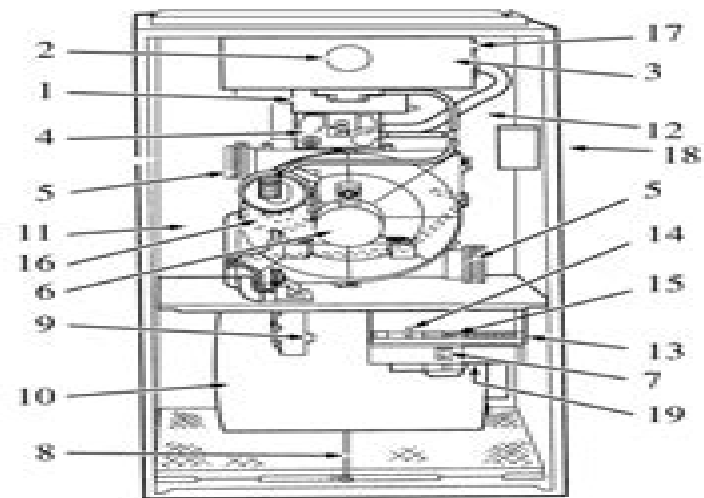
MODELS 340MAV, 350MAV, AND 352MAV FURNACES (UPFLOW POSITION)
