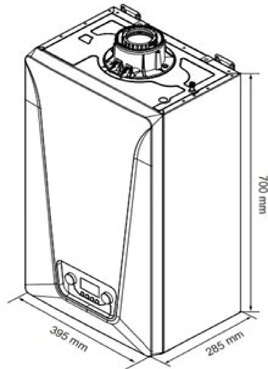
Fig.2 Dimensions and connections
