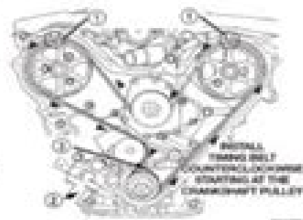
Fig. 78 Timing Belt—Installation
