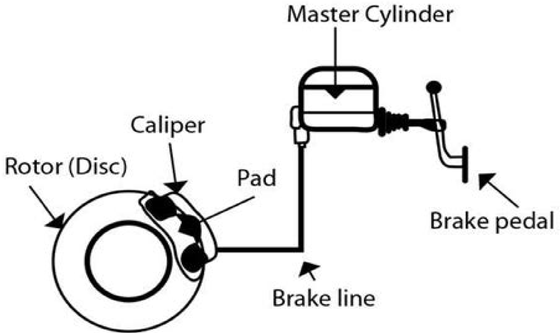
Basic Brake Diagram (Disc brake example)
