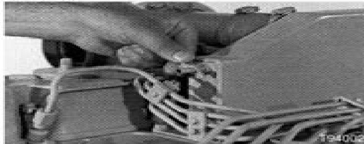
Drain the coolant from the engine. Open the air vent valve on the aftercooler to help drain the coolant.
